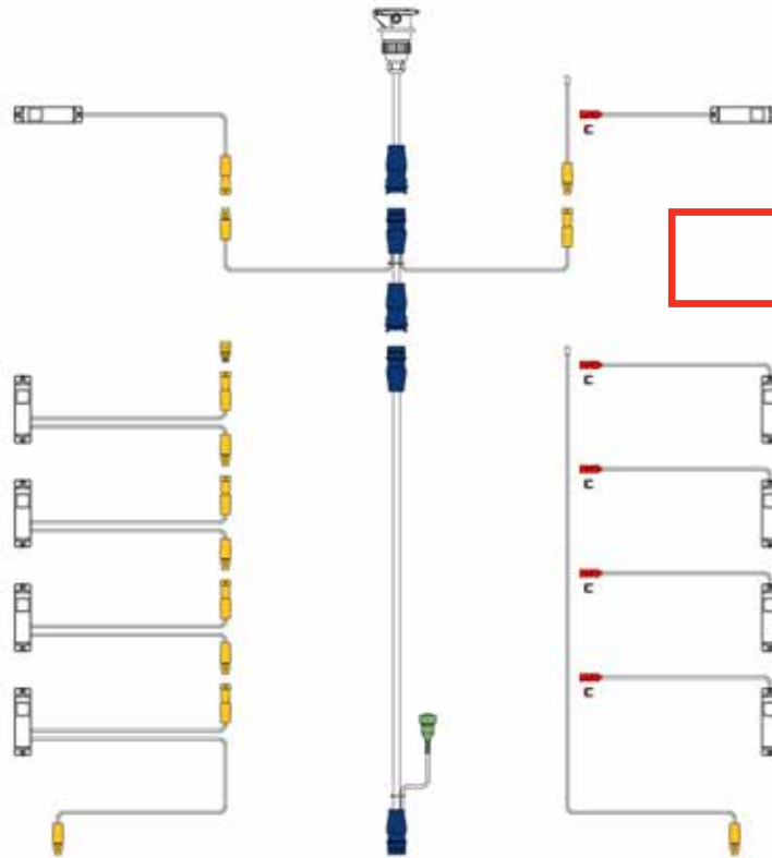
SUPERSEAL wiring system for multi-function light example
