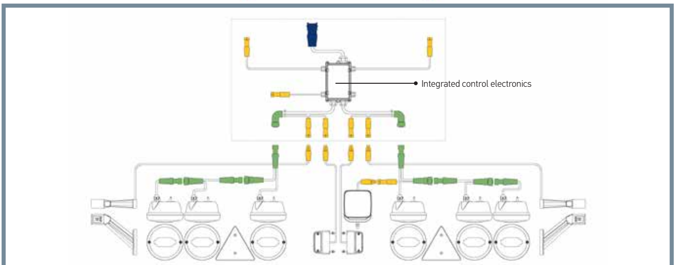
SUPERSEAL wiring system
