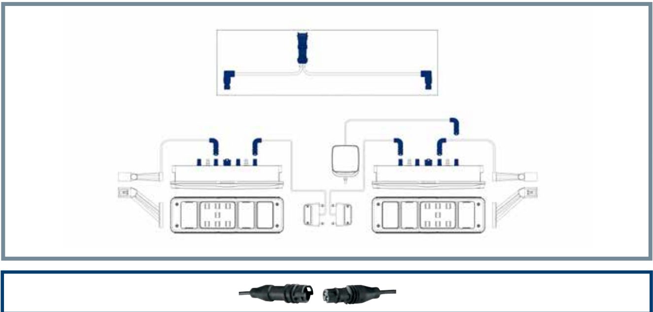
EasyConn wiring system for multi-function light example
